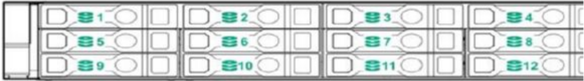
12 LFF + 3 rear LFF drives
